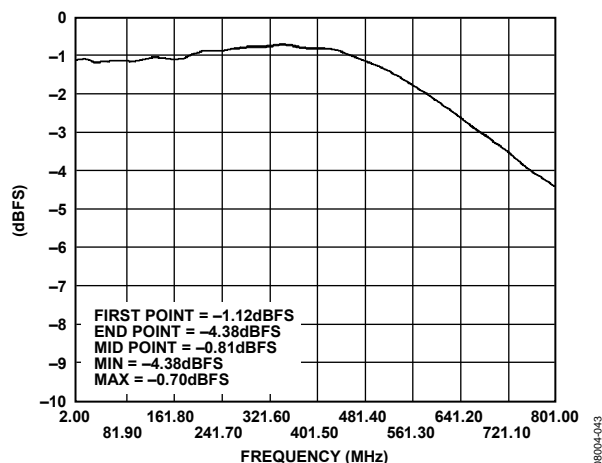
Figure 41. Measured Frequency Response of the Wideband
