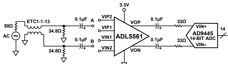
Figure 39. Wideband ADC Interfacing Example Featuring the AD9445
