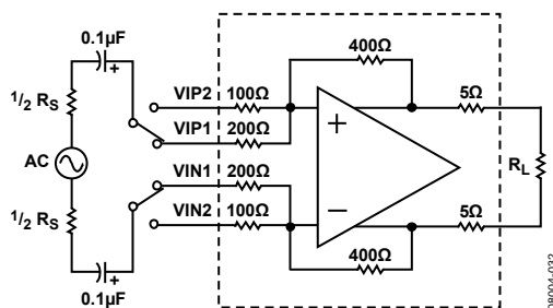
Figure 32. Basic Structure
